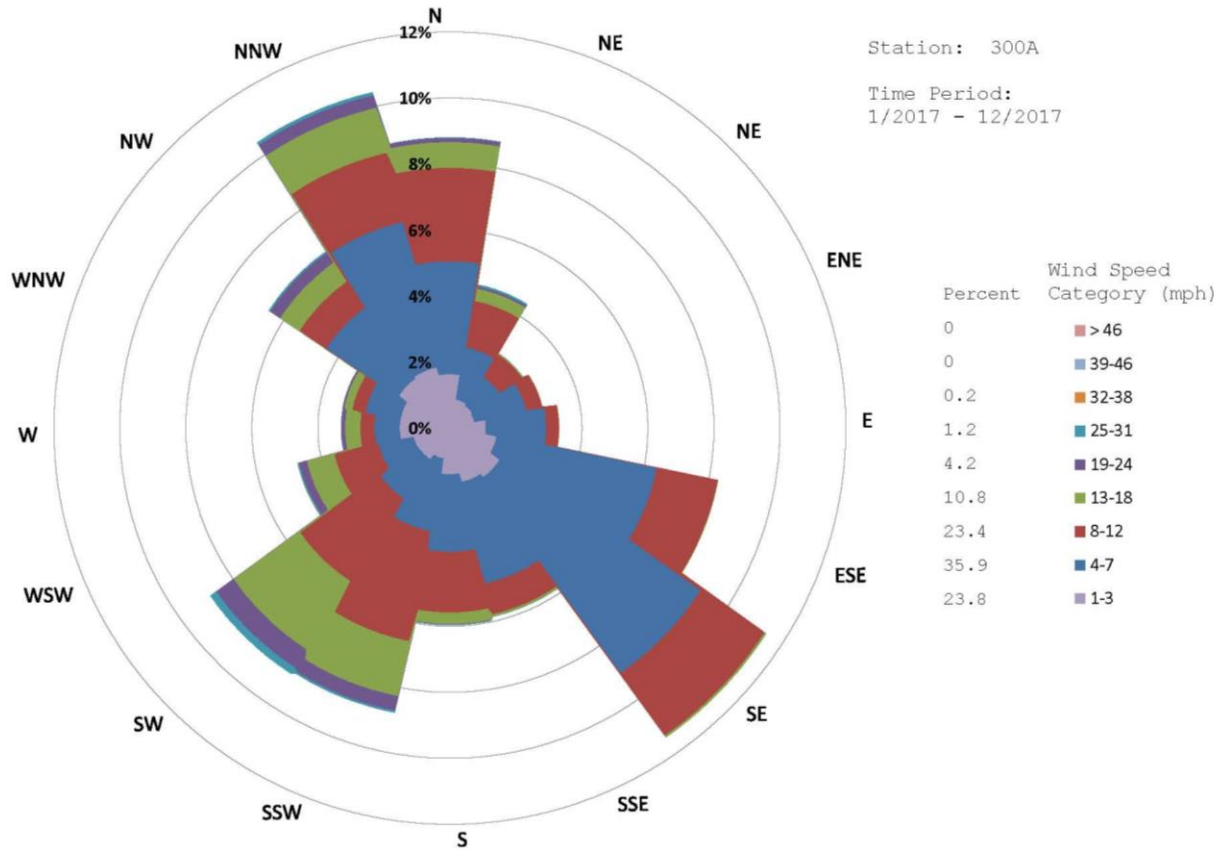
Figure A.1. Hanford Site 300 Area Meteorological Station Wind Rose and Histogram for 2017
